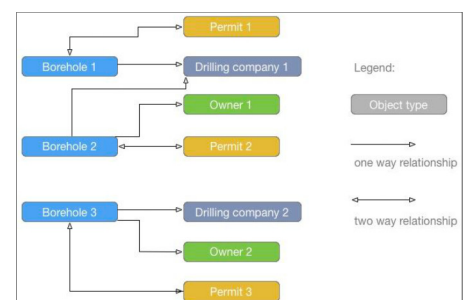
Database design
