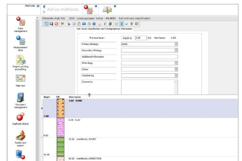
Borehole log with preview window
