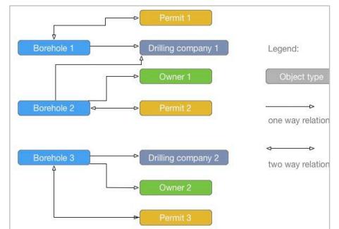
Database design - object relationships
